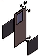
Install gasket bumper and window
